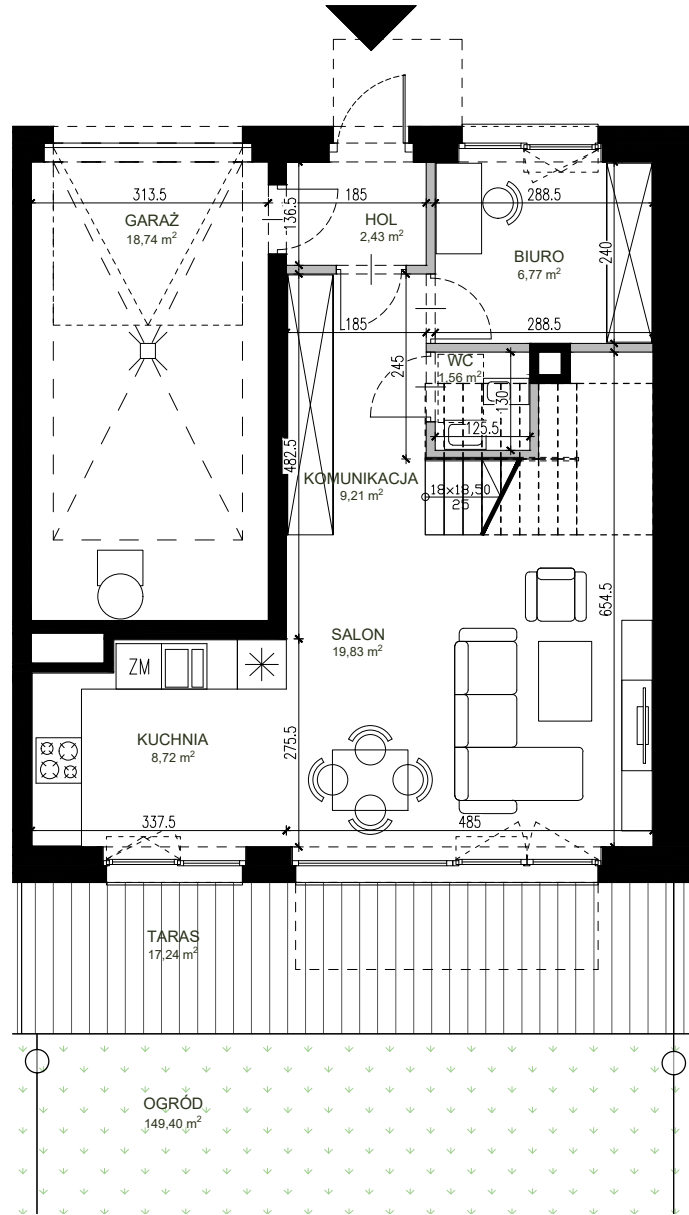
PARTER
